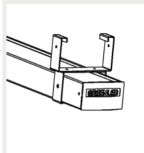
9905214 Omega / ALG2 safety suspensionrail bracket 70
