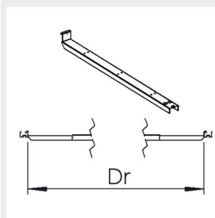
Omega/ALG2 railbracket (4)
